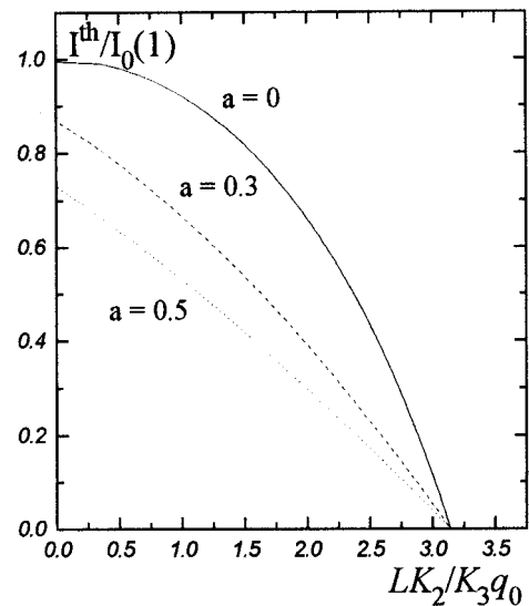
Figure 1. Dependence of the Fréedericksz threshold value on the initial chirality. Here a = (4/\pi^2)(K_2/K_3)\alpha L \tau\delta\chi_{\perp} I_0(1) .
